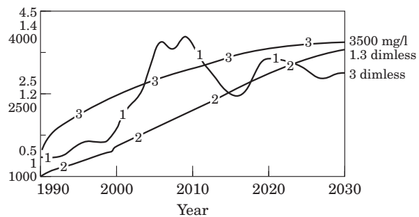
Figure 10. Pesticide, fertilizer and salinization dynamics in the reference behaviour.
